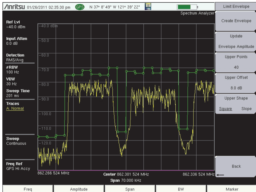
Figure 3-2. Limit Envelope
